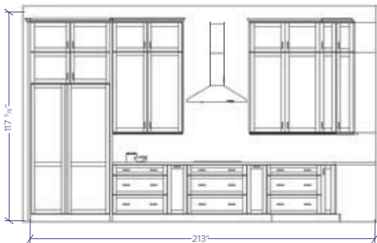
Main Wall Design
